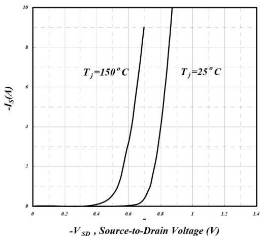
Reverse Diode
