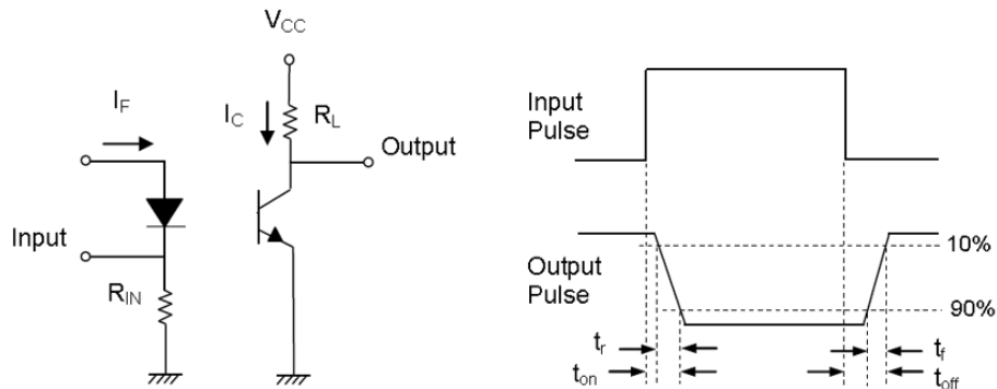
Figure11. Switching Time Test Circuit & Waveforms
