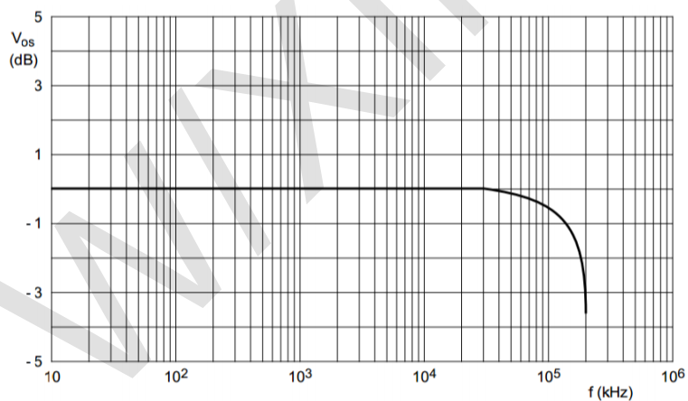
b. Typical frequency response
