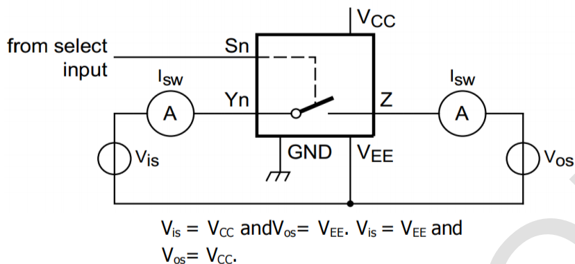
Figure 7. Test circuit for measuring OFF-state current
