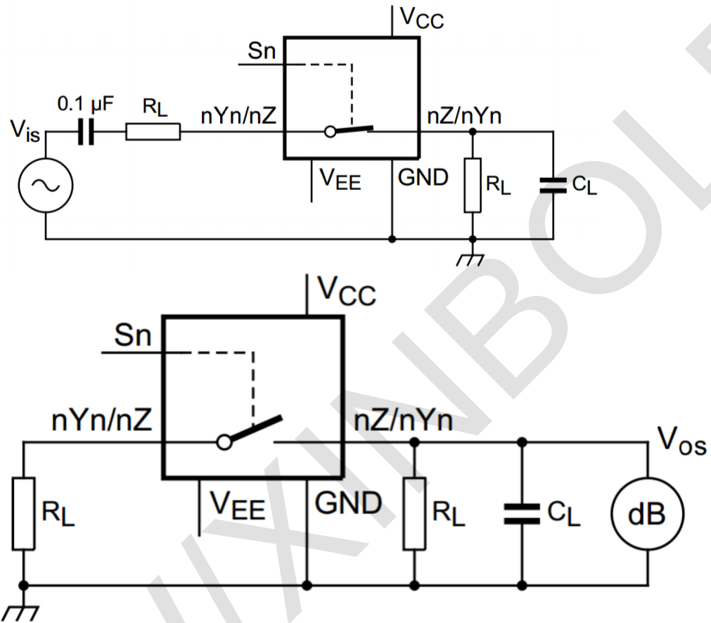
Figure 14. Test circuits for measuring crosstalk between any two switches/multiplexers
