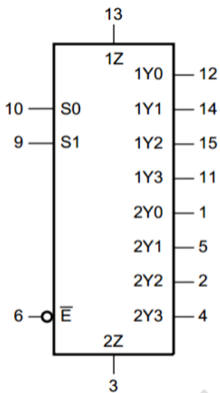
Figure 1. Logic symbol
