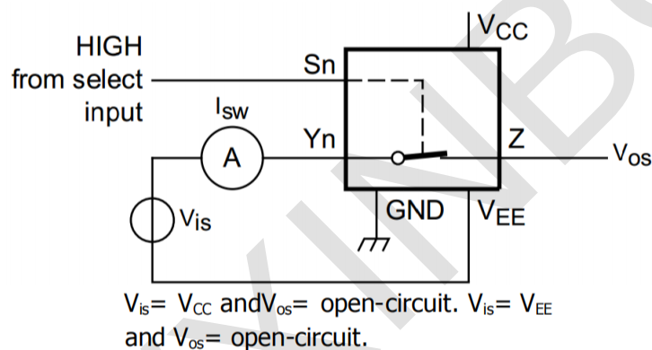
Figure 8. Test circuit for measuring ON-state current
