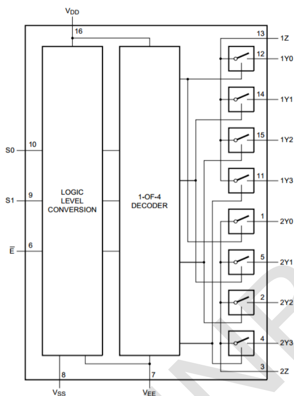
Figure 4. Functional diagram
