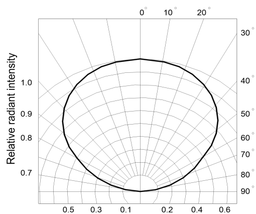
Fig.6 Radiation diagram
