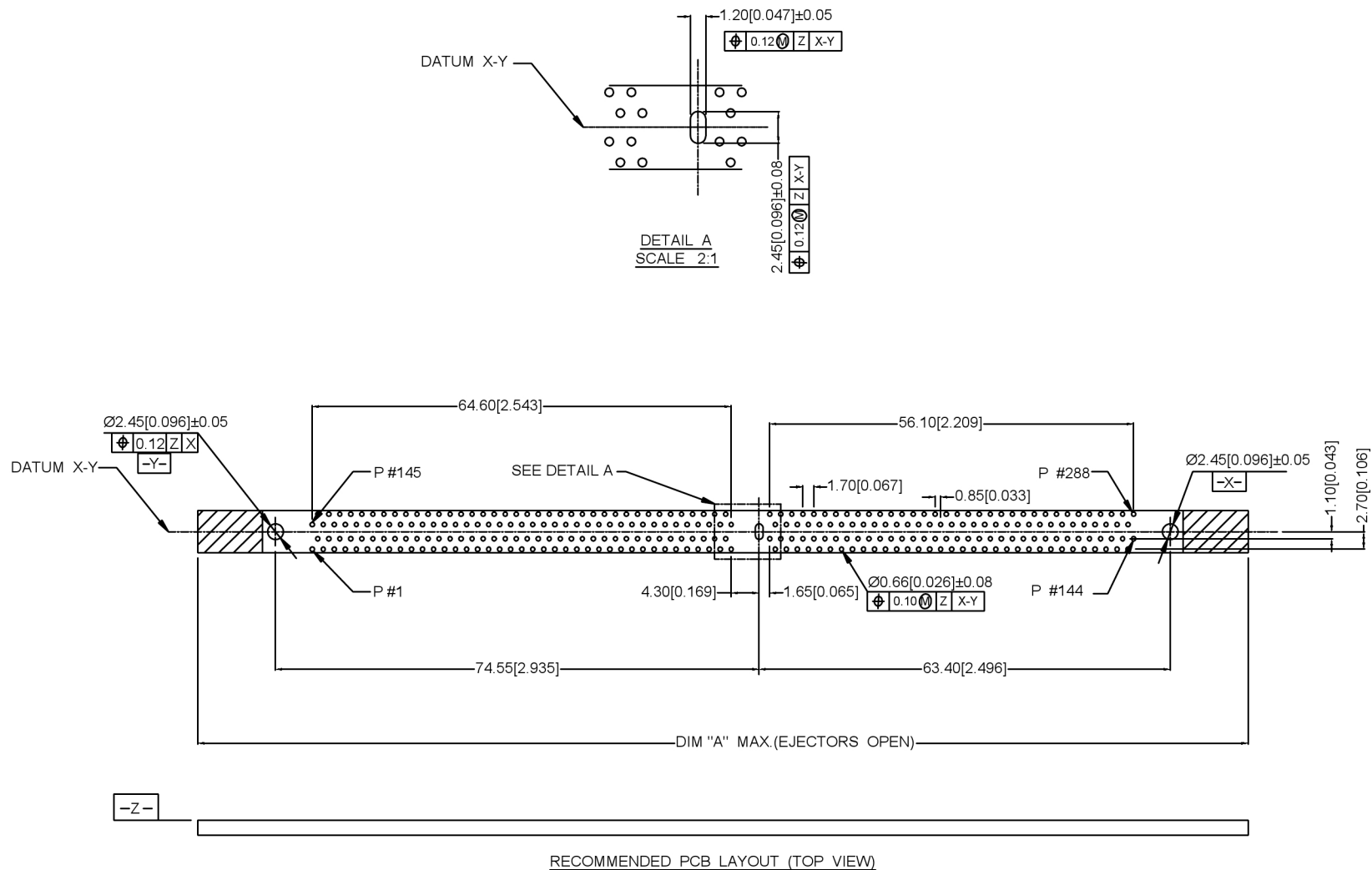
RECOMMENDED PCB LAYOUT (TOP VIEW)
