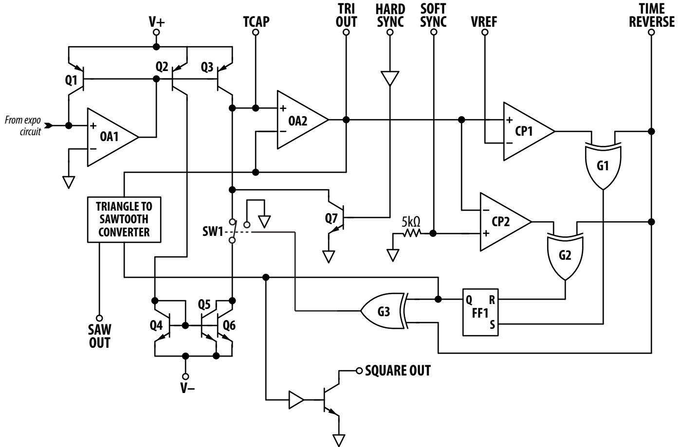
Figure 11: SSI2130 Simplified Oscillator Core
