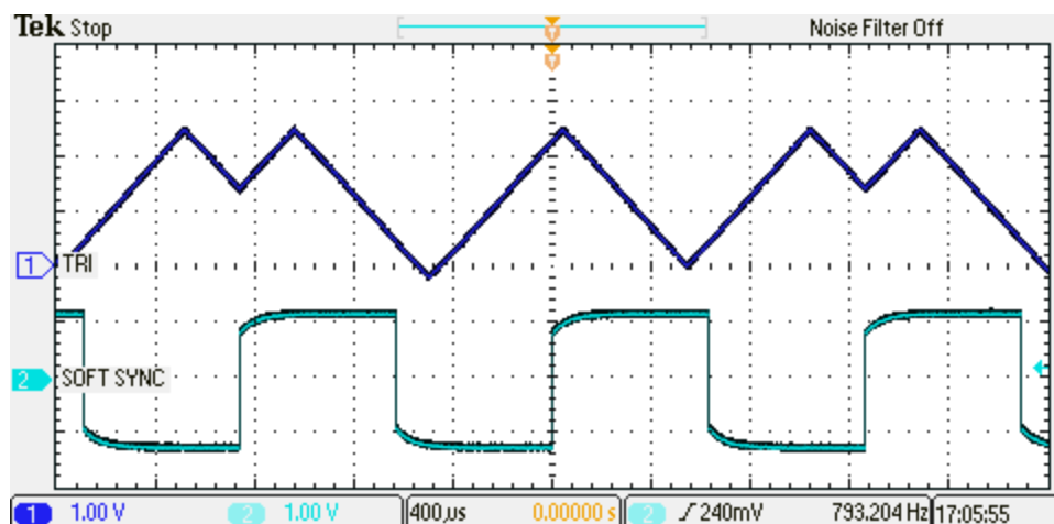
Figure 4: “Soft” Sync
