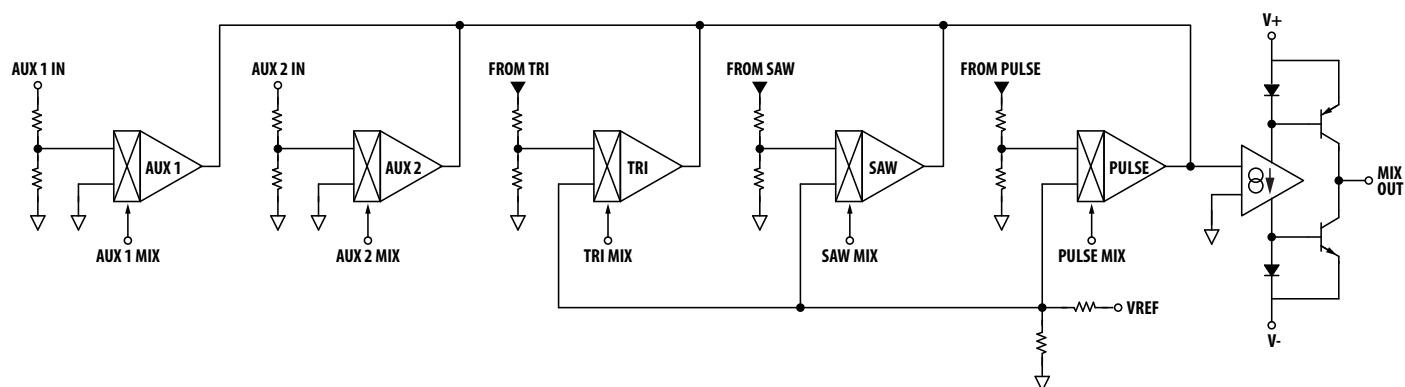
Figure 14: Mixer Section
