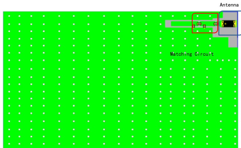
Figure 2. MAN6090C32 PCB Layout (Unit: mm) TOP VIEW:
