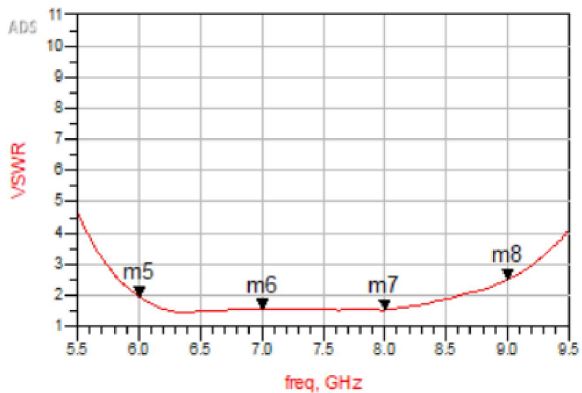
Figure 6. MAN6090C32 VSWR
