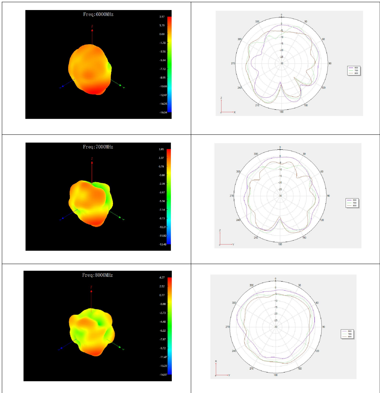
Figure 9. Radiation Pattern
