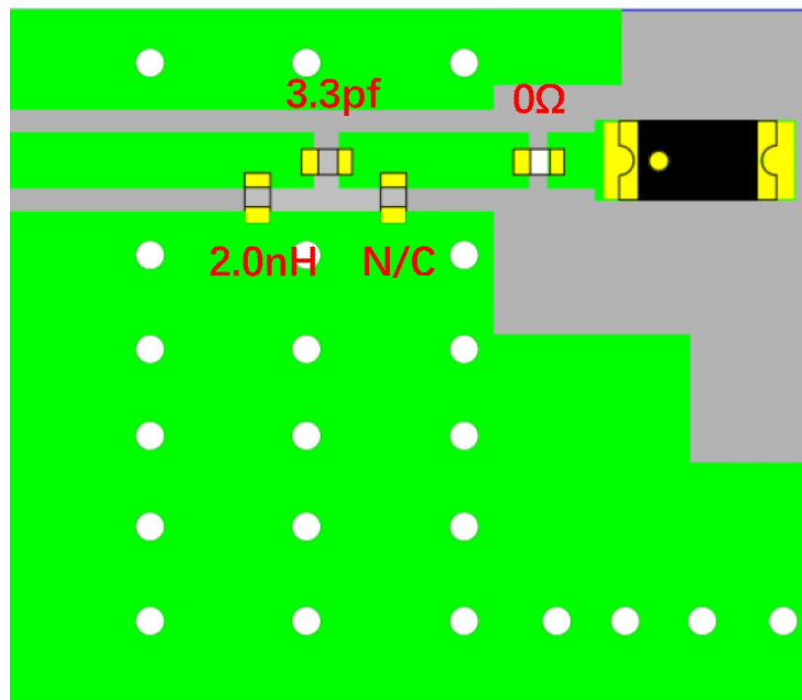
Figure 5. MAN6090C32 Matching Circuit (Unit: mm)
