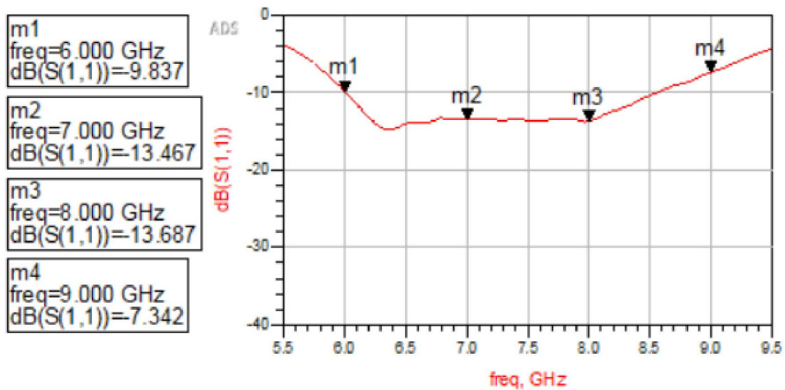
Figure 7. MAN8060 Return Loss
