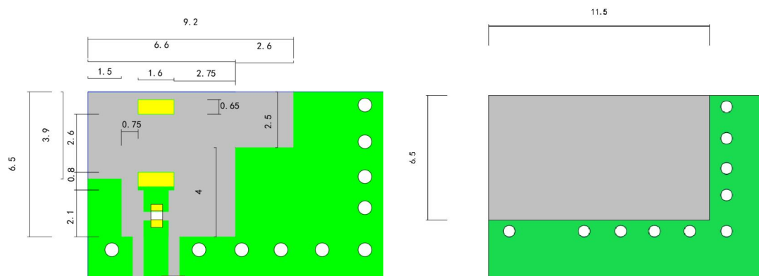
Figure 4. MAN6090C32 PCB Antenna Layout (Unit: mm)
