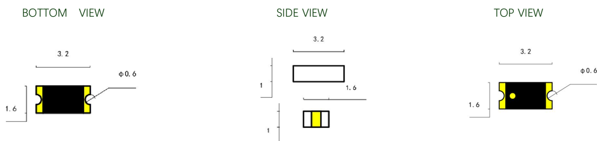
Figure 1. MAN6090C32 View (Unit: mm)
