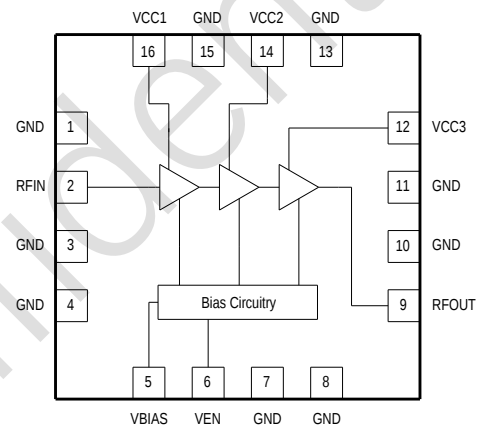
Figure 2. GDM3728 Function Block Diagram
