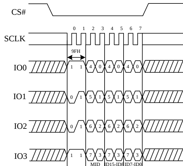
Figure 12. Read Identification ID Sequence Diagram (QPI)
