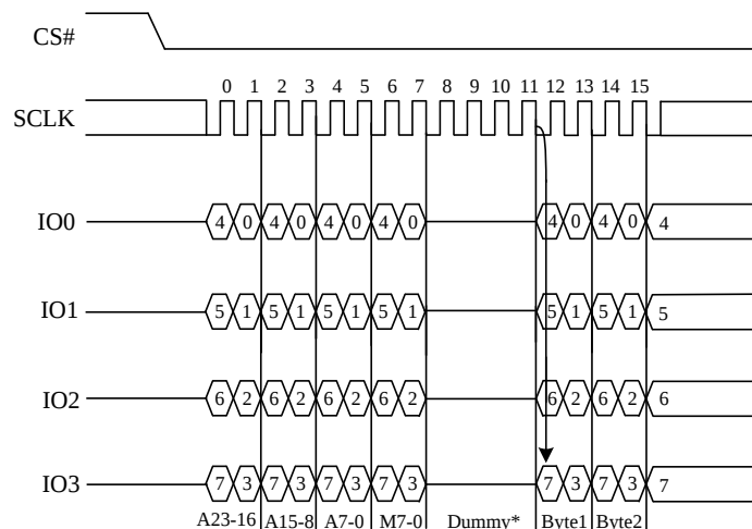
Figure 21. Quad I/O Fast Read Sequence Diagram (M5-4=(1,0))
