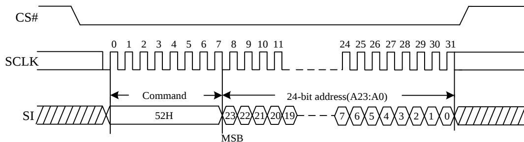
Figure 37. 32KB Block Erase Sequence Diagram
