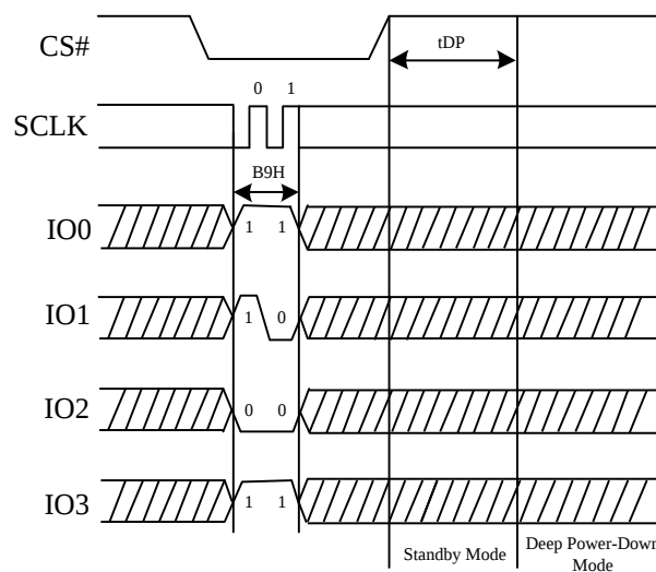
Figure 61. Deep Power-Down Sequence Diagram (QPI)
