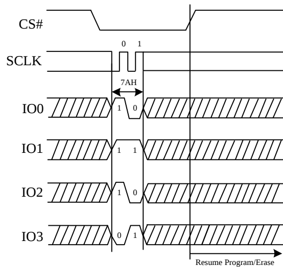
Figure 54. Program/Erase Resume Sequence Diagram (QPI)
