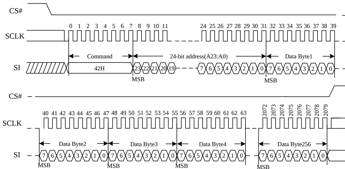
Figure 68. Program Security Registers command Sequence Diagram
