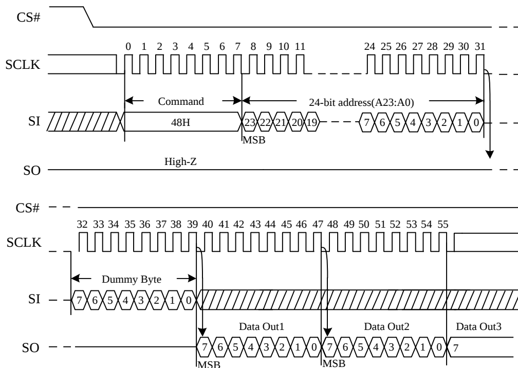
Figure 70. Read Security Registers command Sequence Diagram
