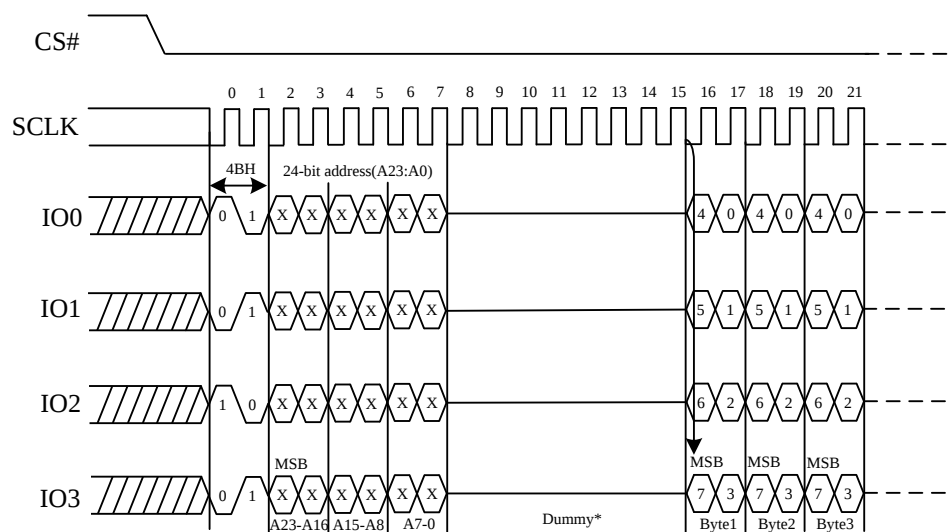
Figure 10. Read Unique ID (RUID) Sequence (QPI)
