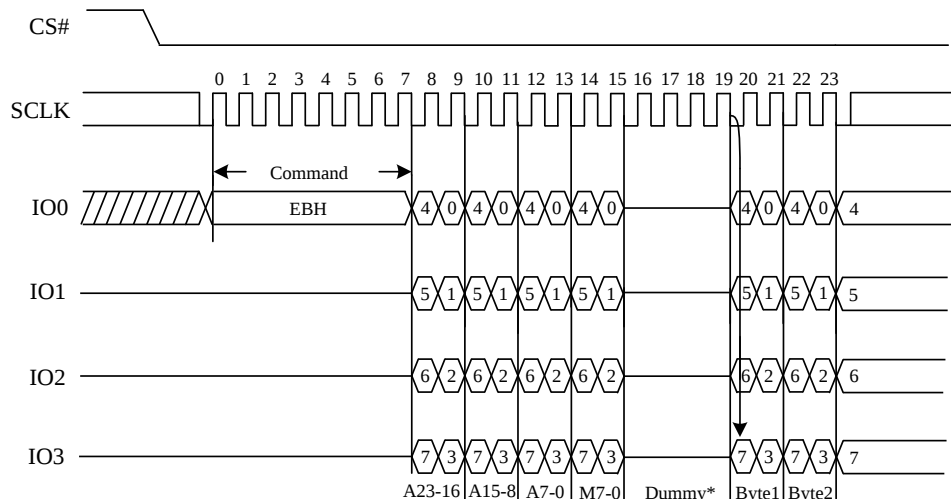
Figure 20. Quad I/O Fast Read Sequence Diagram (M5-4=(1,0))
