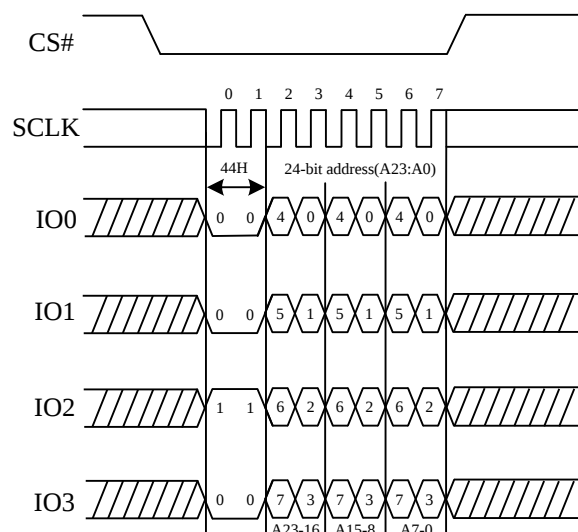
Figure 67. Erase Security Registers command Sequence Diagram (QPI)
