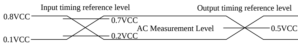
Figure 74. Absolute Maximum Ratings Diagram
