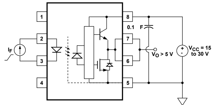
Figure 19. I_{FIH} Test circuit.
