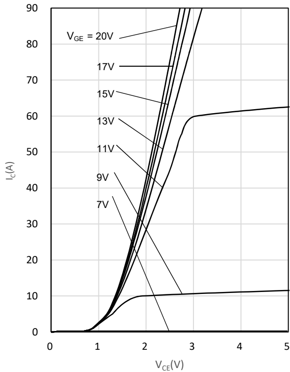
Fig. 5 Output characteristics
