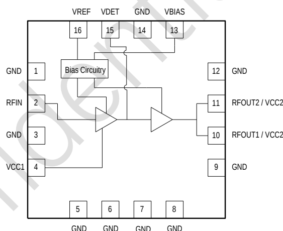
Figure 2. GSM1820 Function Block Diagram
