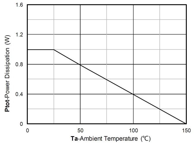
Power dissipation
