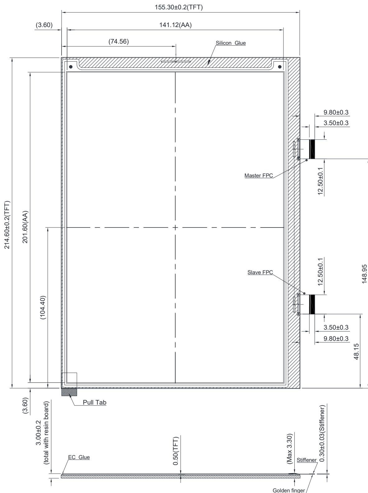
Figure 1-1 EPD Drawing
