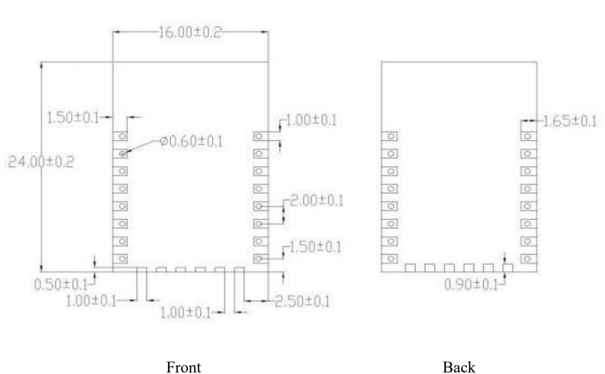
Figure 4 Dimension diagram
