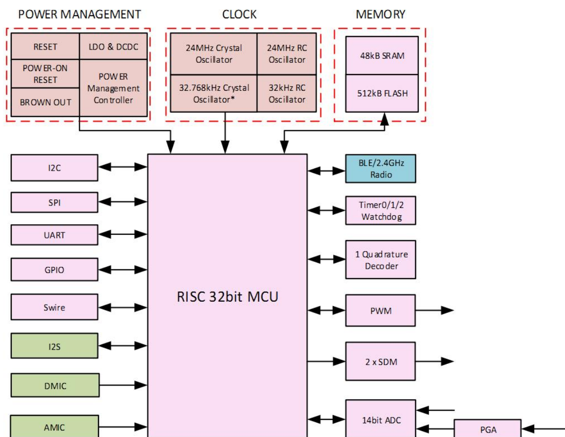
Figure 1 Main chip architecture diagram
