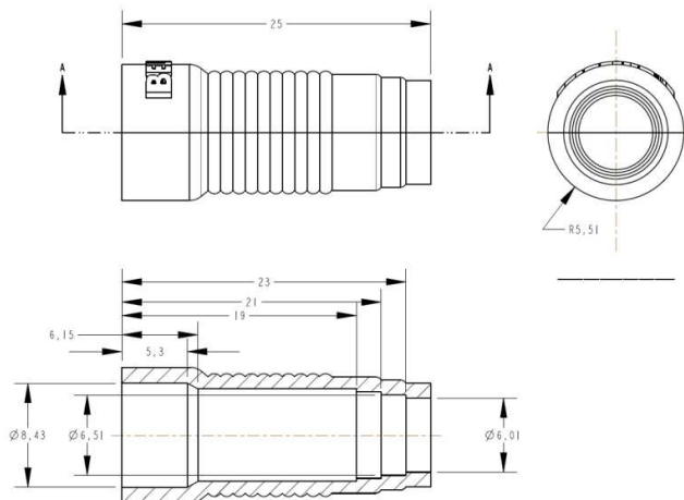
Figure 1 – SLS-59/6 with dimensions
