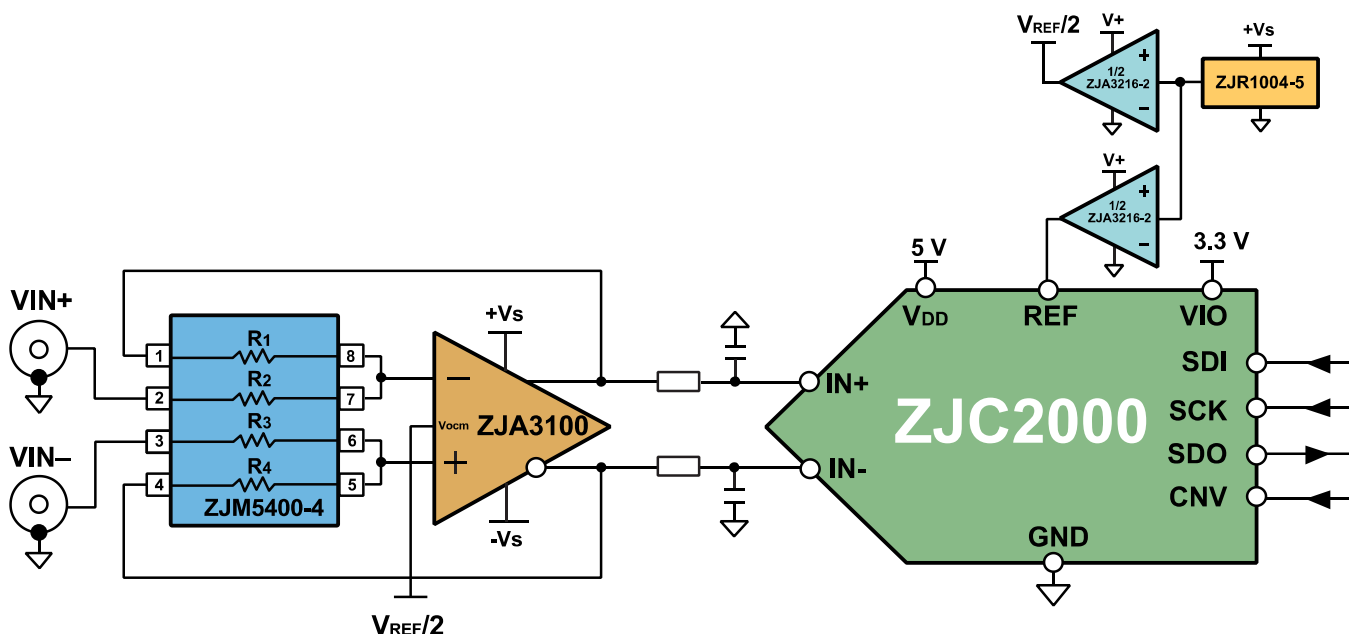
Figure 22. Using ZJA3100 with 18-bit SAR ADC ZJC2000
