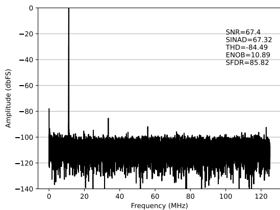
(a) 输入信号频率 = 11MHz
