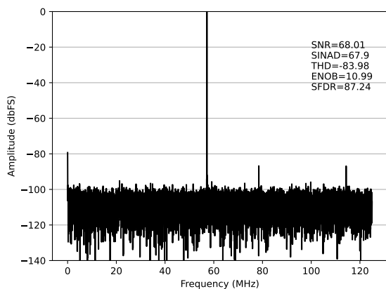
(c) 输入信号频率 = 57MHz
