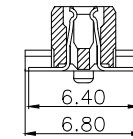
SECTION: A-A 7.7H/11.7H/15.7H
