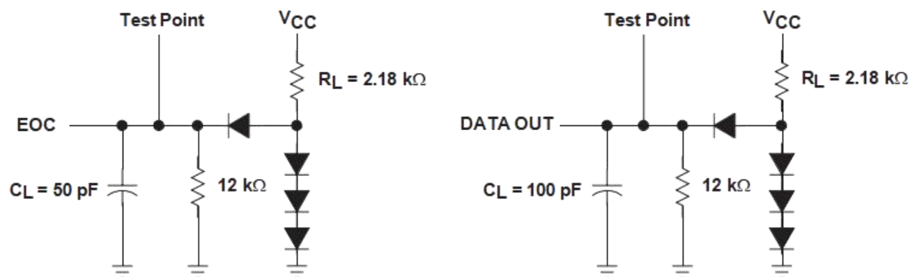
Figure 2. Load Circuits
