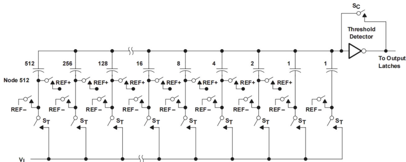
Figure 1. Simplified Model of the Successive-Approximation System chip-select operation
