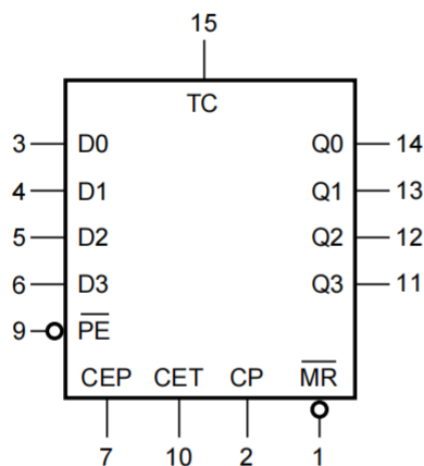
Figure 1. Logic symbol
