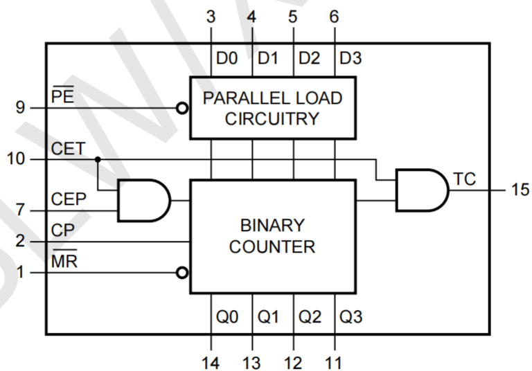
Figure 3. Functional diagram
