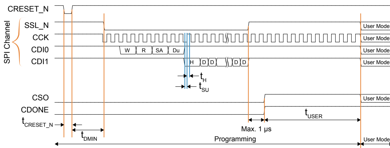
Figure 50: SPI Active (x1) Timing Sequence
