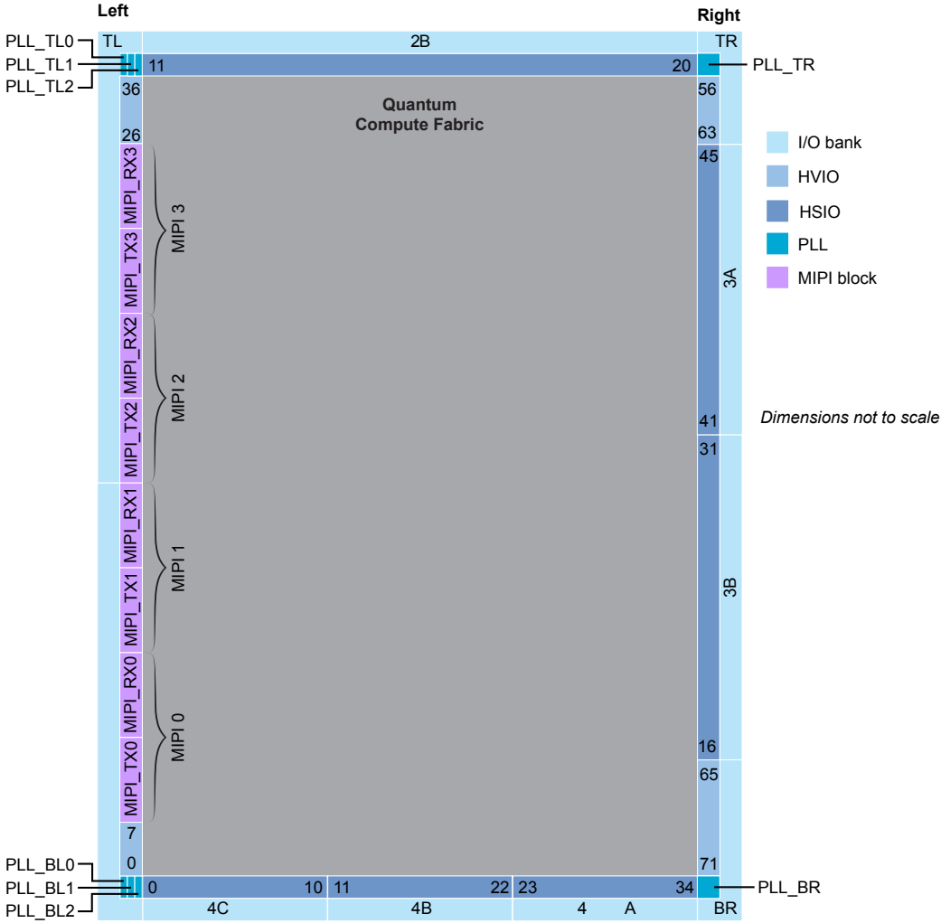
Figure 54: Floorplan Diagram for L484 Packages
