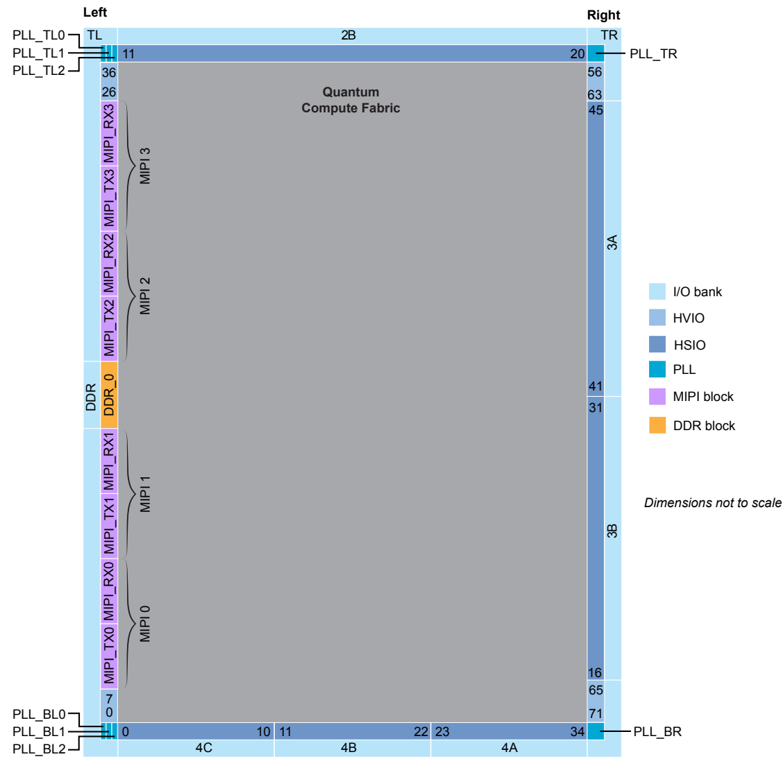
Figure 55: Floorplan Diagram for J484 and M484 Packages
