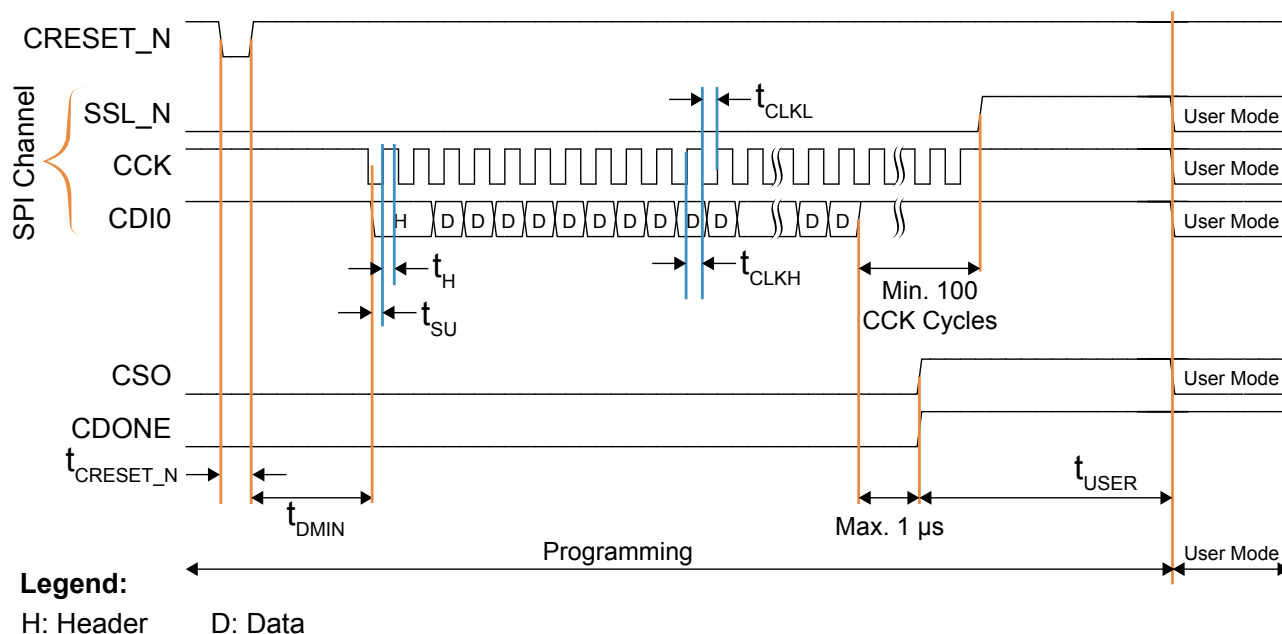
Figure 51: SPI Passive Mode (x1, Mode 3) Timing Sequence
