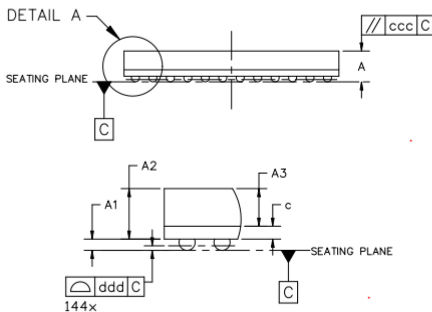
Fig. 2-4 RK628H Package Side View
