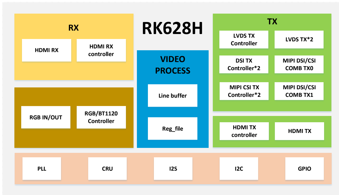
Fig. 1-1 RK628H Block Diagram
