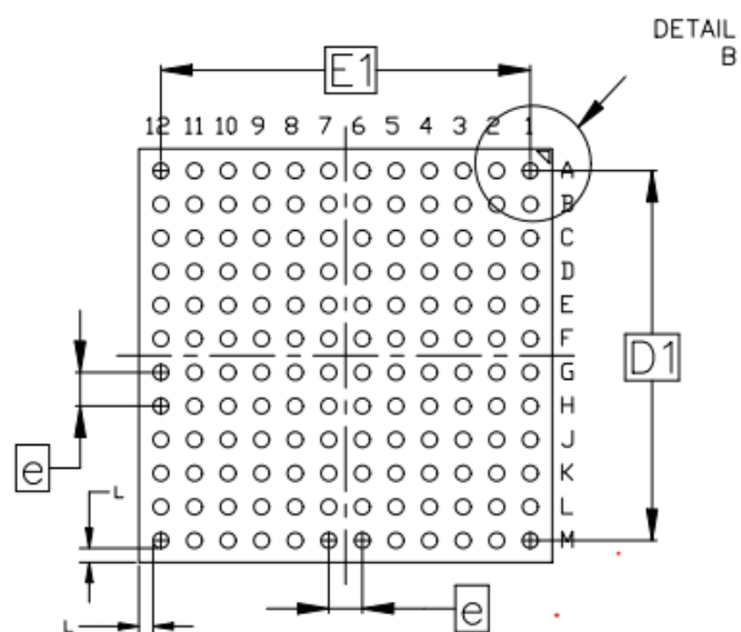
Fig. 2-3 RK628H Package Bottom View
