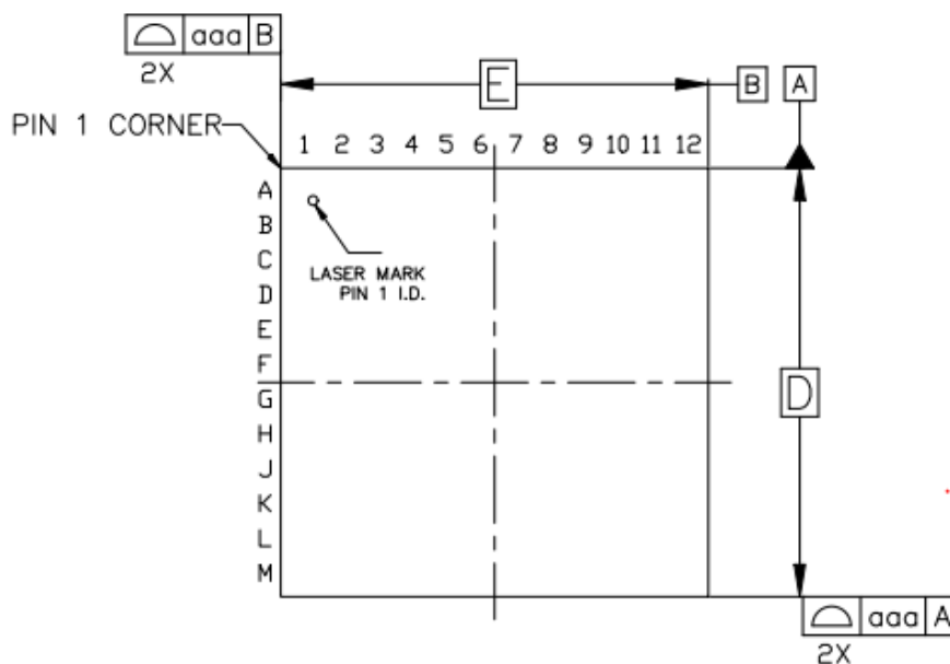
Fig. 2-2 RK628H Package Top View
