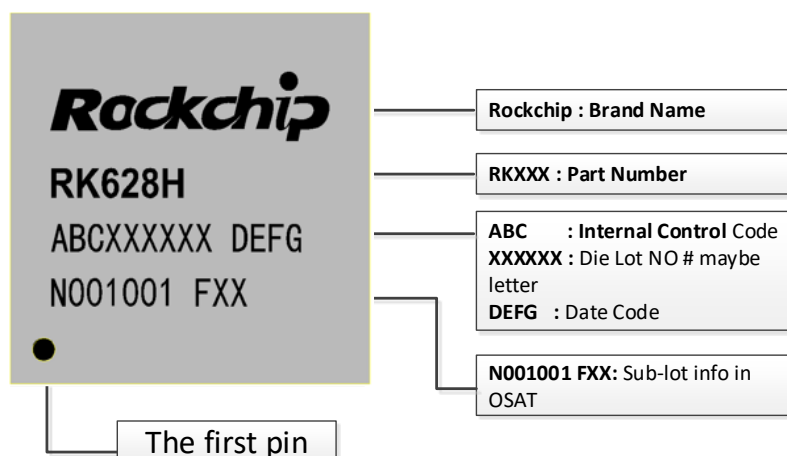
Fig. 2-1 RK628H Package Definition
