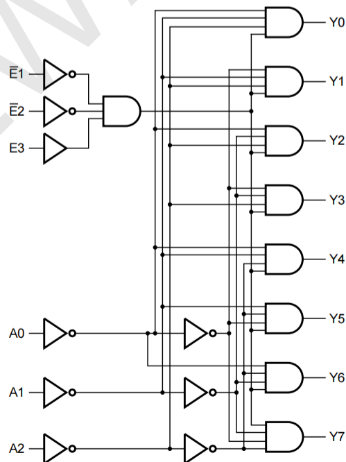
Figure 3. Logic diagram
