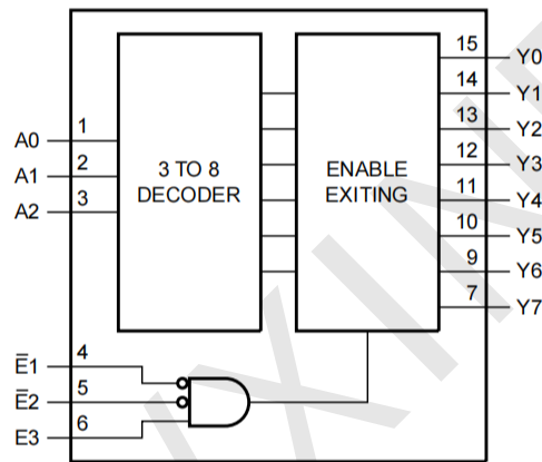
Figure 2. Functional diagram
