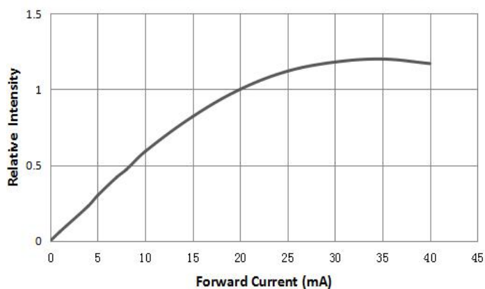
Relative Intensity VS. Forward Current ( T_a=25^{\circ}\text{C} )
