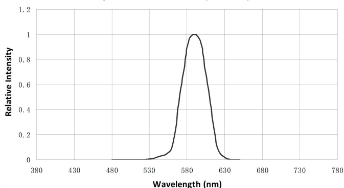
Spectrum Distribution ( T_a=25^{\circ}\text{C} )
