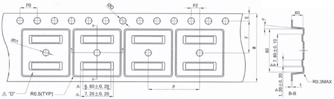
Figure 21.16-16-Lead Narrow Body SOIC [NB SOIC-16] Reel Information—dimension unit(mm)
