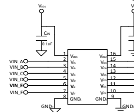
Figure 1. \pi 160xxx/\pi 161xxx/\pi 162xxx/\pi 163xxx functional Block Diagram
