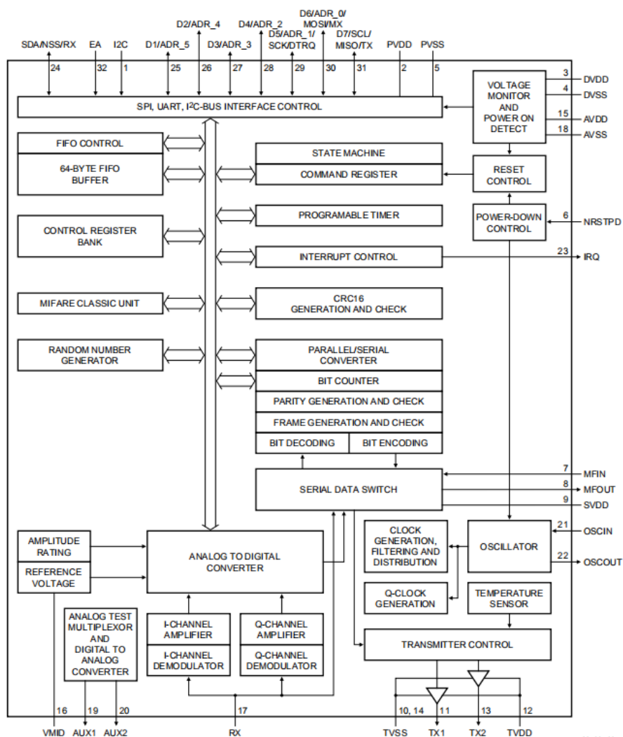
Figure 4-2 Detailed block diagram of the Si522A
