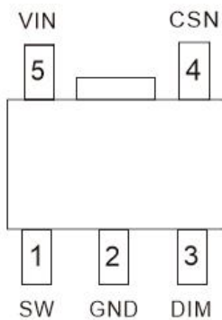
D3815C-TD(SOT89-5)
