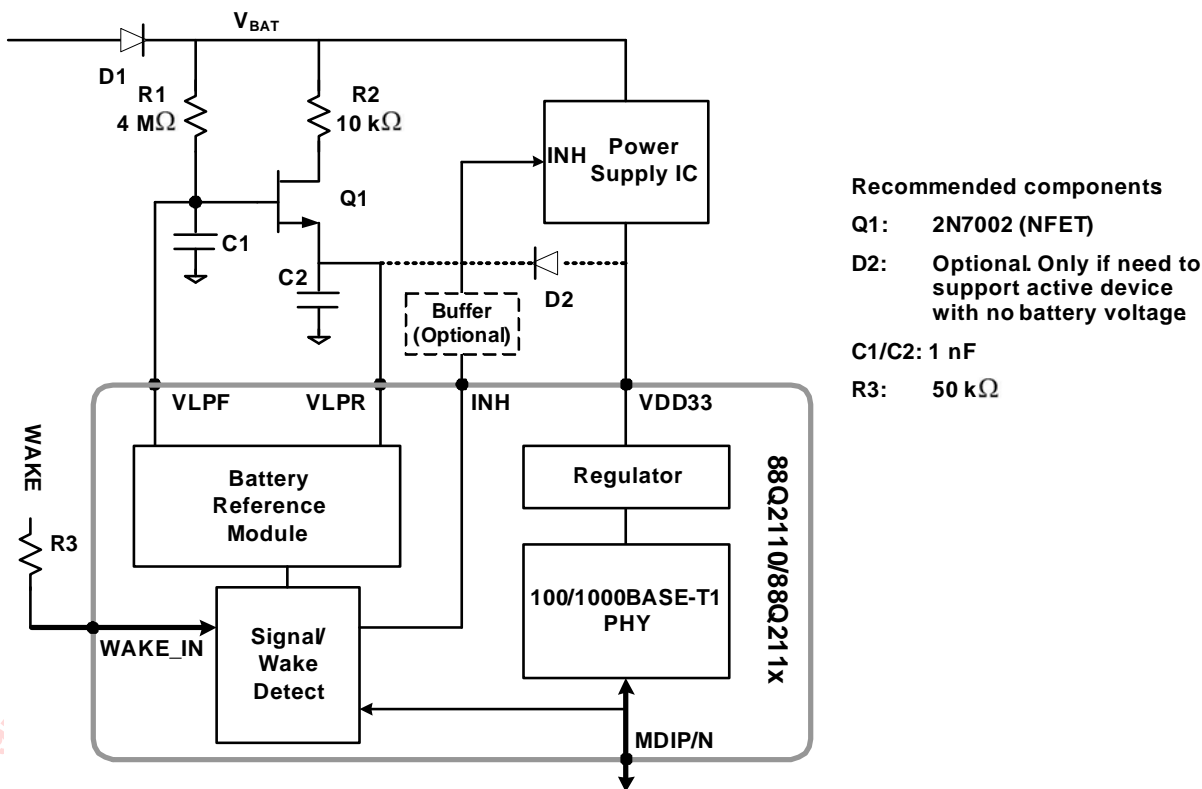
Figure 9: LPSD Block Diagram
