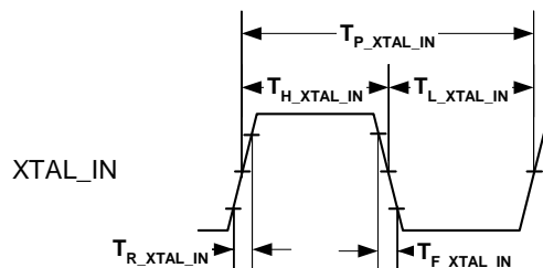
Figure 25: XTAL_IN/XTAL_OUT Timing
