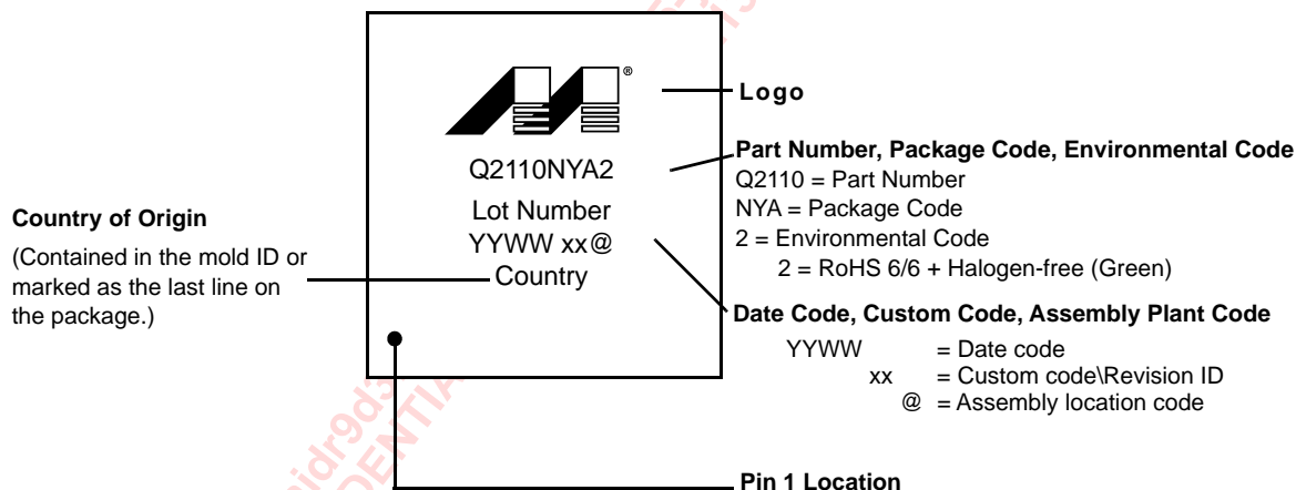
Figure 39: 88Q2110 40-pin QFN Sample Package Marking and Pin 1 Location
