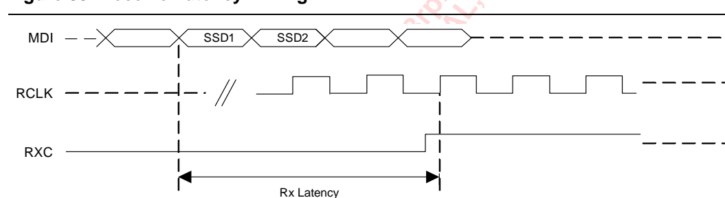
Figure 35: Receive Latency Timing
