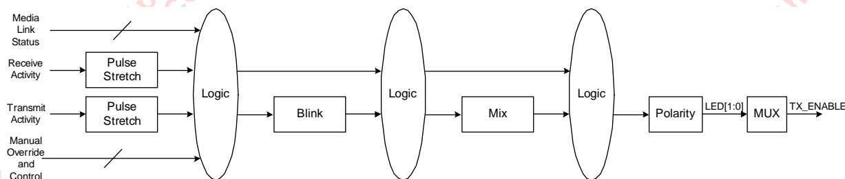
Figure 13: LED Chain
