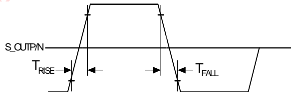
Figure 32: Serial Interface Rise and Fall Time
