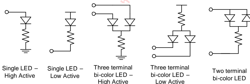
Figure 14: Various LED Hookup Configurations
