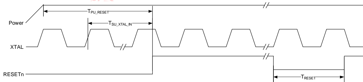
Figure 24: Reset Timing
