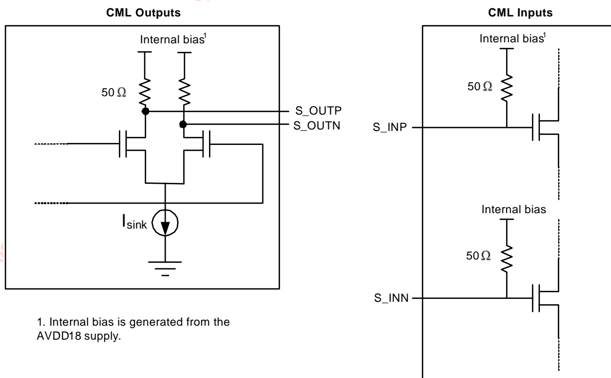
Figure 5: CML I/Os
