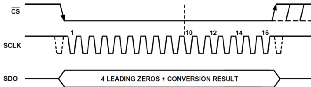
Figure 4. Timing Diagram
