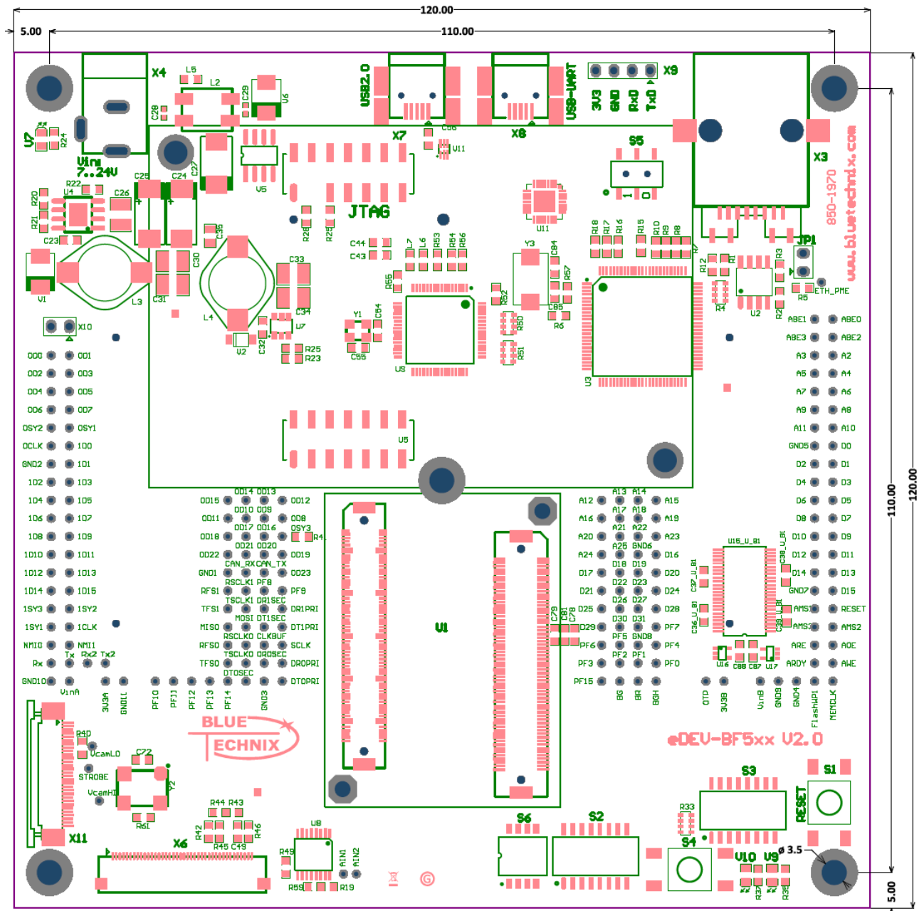
Figure 6-1: Mechanical outline top view
