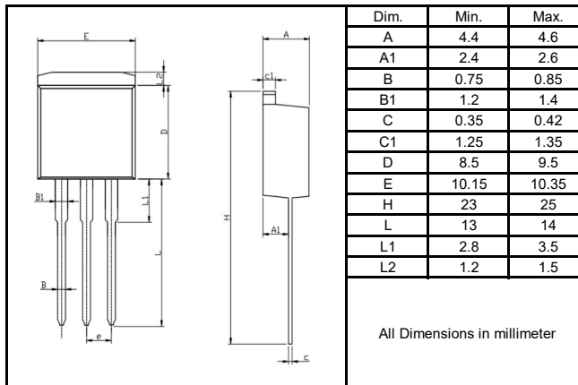
T0-262
