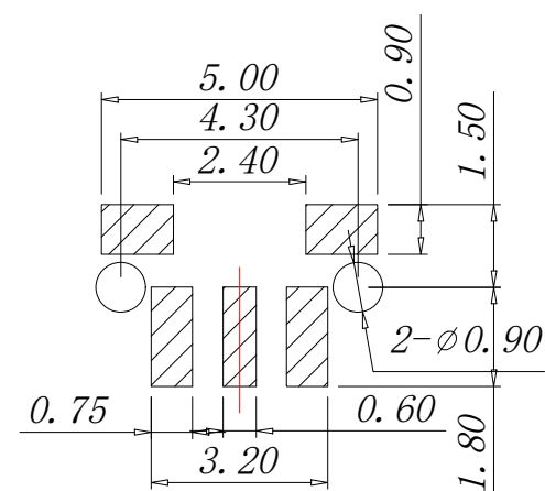
PCB.WELDING DRAWING
