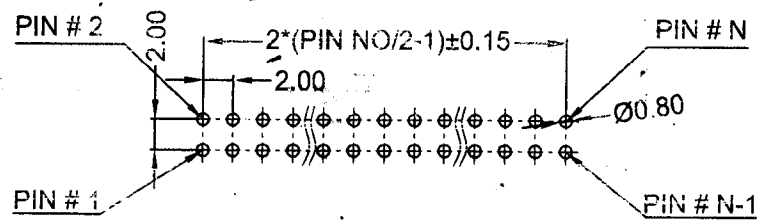
P.C.B. LAYOUT(TOP VIEW) TOLERANCE:±0.05
