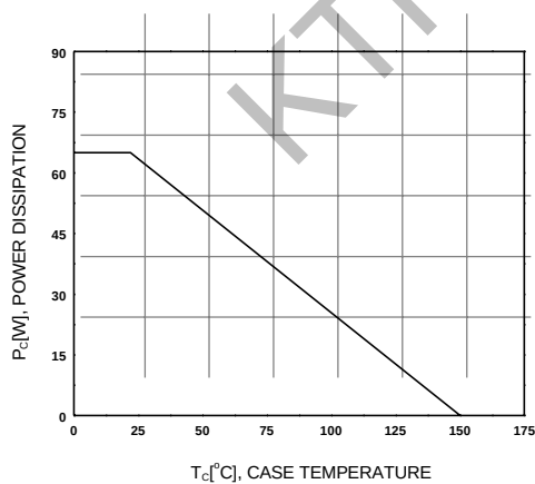
Figure 5. Power Derating
