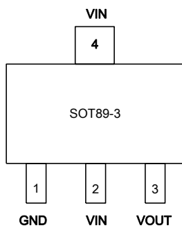
LP3994-XXX3F (top view)
