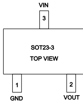
LP3994-XXB3F (top view)
