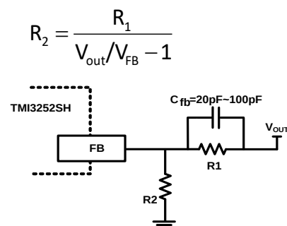
Figure 2. Feedback Network
