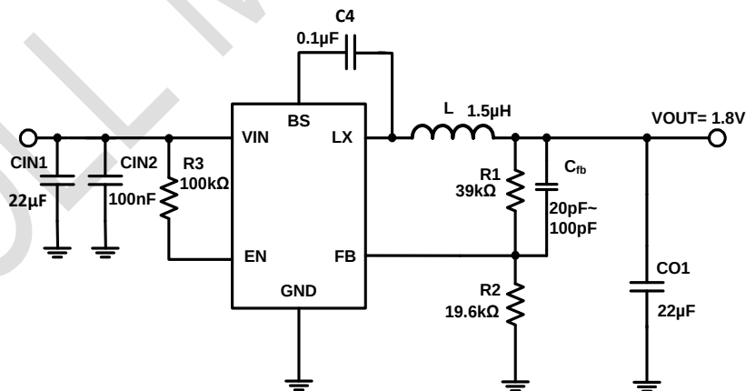
Figure 6. 12V IN , 1.8V Output ( V_{FB}=0.6V )
