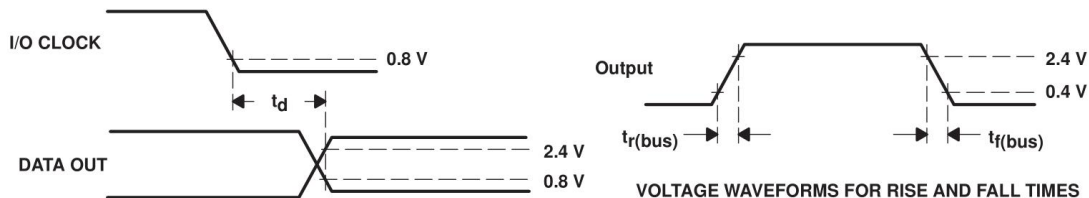
VOLTAGE WAVEFORMS FOR RISE AND FALL TIMES
