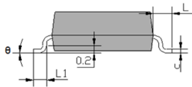
Package outline : SOD-123
