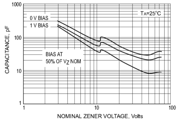
Typical Capacitance
