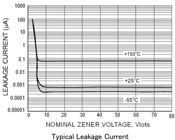
Typical Leakage Current
