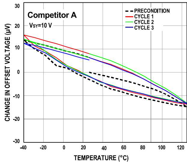
Figure 46. Competitor A Offset Voltage over Three Full Temperature Cycles
