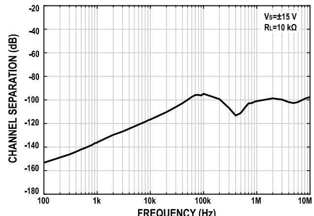
Figure 24. Channel Separation vs. Frequency
