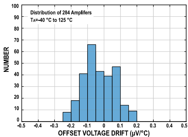
Figure 8. Offset Voltage Drift Distribution (-40 °C to 125 °C)
