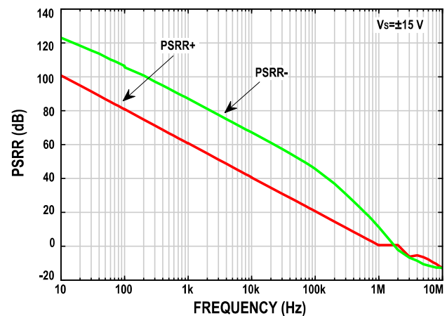
Figure 20. Power Supply Rejection Ratio (PSRR) vs. Frequency
