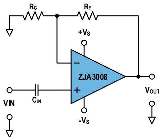
Figure 43. Incorrect AC-Coupled Op Amp Circuit
