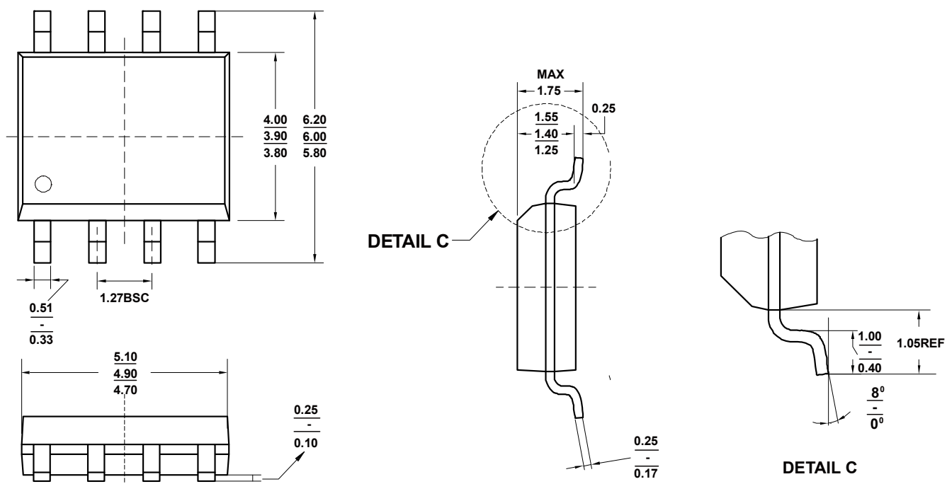
Figure 50. 8-Lead SOIC Package Dimensions shown in millimeters
