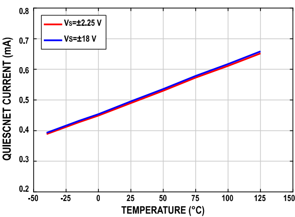
Figure 27. Quiescent Current vs. Temperature
