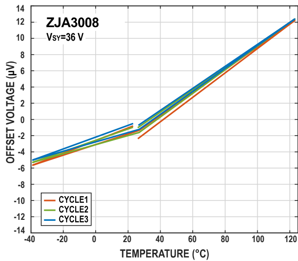
Figure 45. ZJA3008 Offset Voltage over Three Full Temperature Cycles
