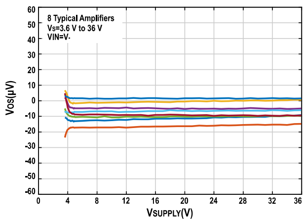
Figure 12. Offset Voltage vs. Power Supply, V IN =V -
