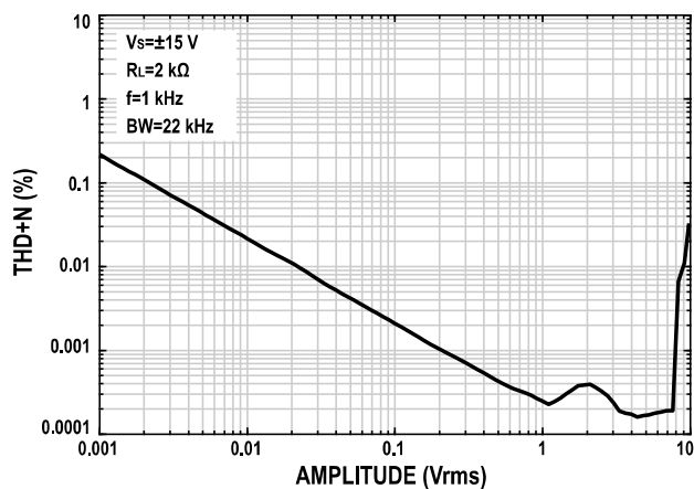
Figure 36. THD+N vs. Amplitude
