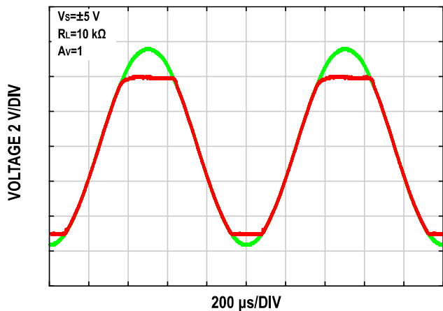
Figure 42. ZJA3008 Has No Output Phase Reversal
