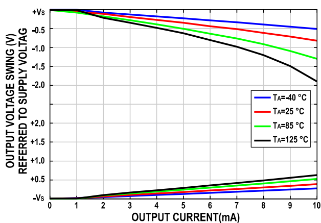
Figure 34. Output Voltage Swing vs. Output Current
