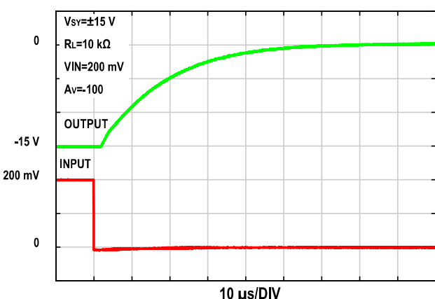
Figure 21. Positive Overload Recovery
