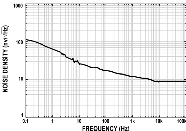
Figure 25. Voltage Noise Density vs. Frequency
