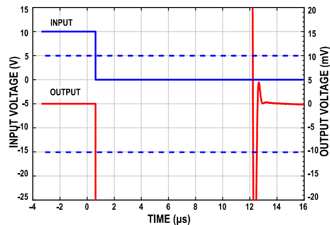
Figure 29. Settling Time
