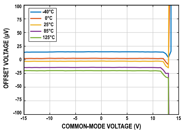
Figure 10. Offset Voltage vs. Common-Mode Voltage
