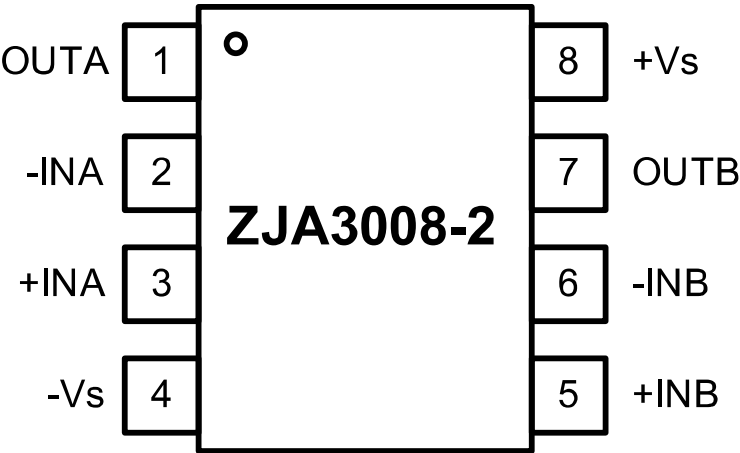
Figure 1. ZJA3008-2 Pin Configuration (8-lead SOIC and MSOP)
