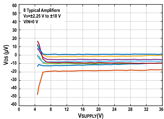
Figure 11. Offset Voltage vs. Power Supply, V IN =0 V
