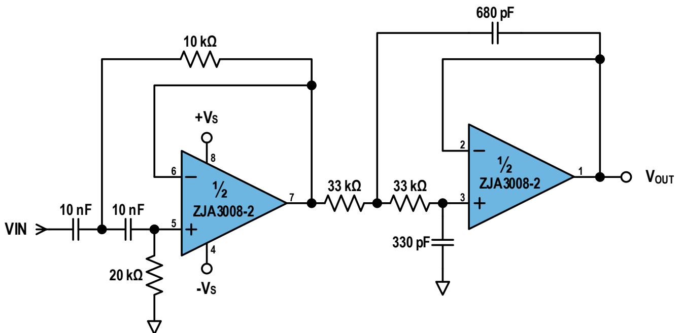
Figure 49. Using ZJA3008-2 to Build a 2-stage Band-pass KRC Filter
