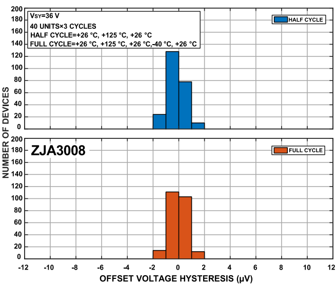
Figure 47. Histogram Showing the ZJA3008's Temperature Hysteresis of the Offset Voltage over Three Full Cycles and over Three Half Cycles
