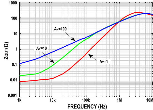
Figure 31. Closed-Loop Output Impedance
