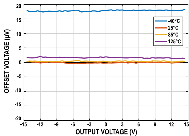
Figure 13. Offset Voltage vs. Output Voltage, R L =10 kΩ
