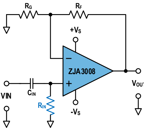
Figure 44. Creating an Input Bias Current Return Path
