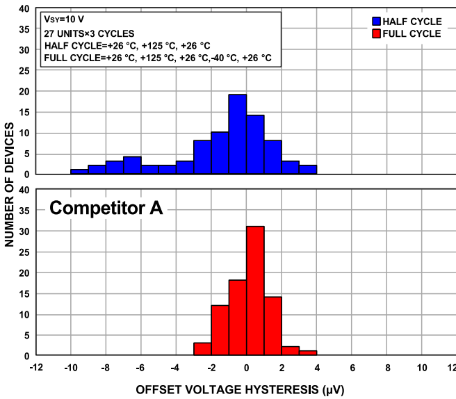
Figure 48. Histogram Showing the Competitor A's Temperature Hysteresis of the Offset Voltage over Three Full Cycles and over Three Half Cycles
