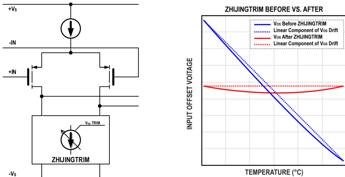
Figure 40. Diagram of Post-package Trimming Scheme (Left) and Effect (Right)
