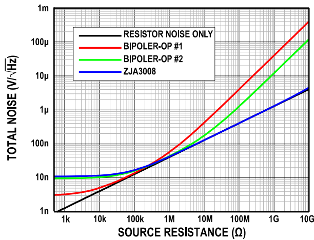
Figure 41. System Total Noise vs. Source Impedance
