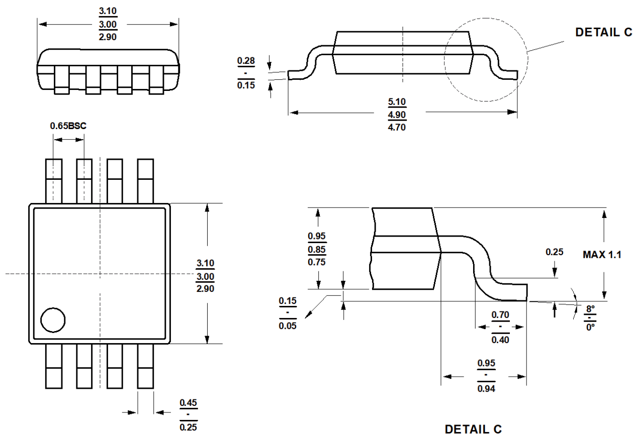
Figure 51. 8-Lead MSOP Package Dimensions shown in millimeters
