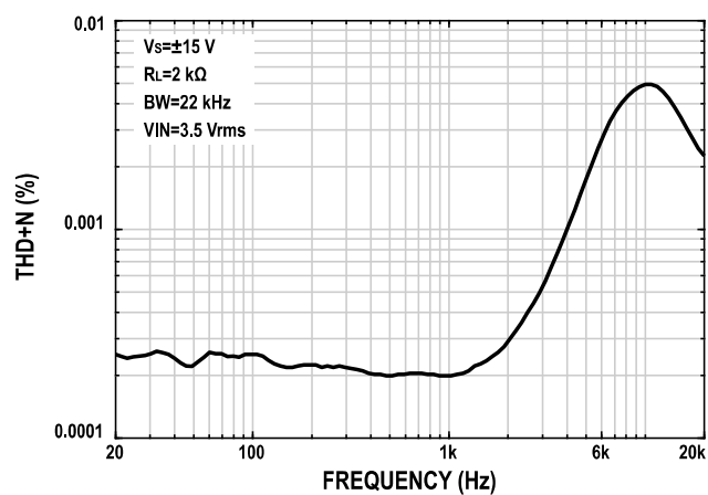
Figure 35. THD+N vs. Frequency
