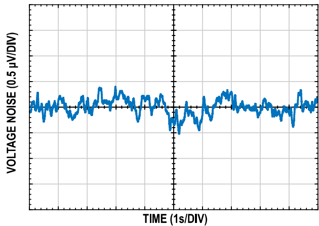
Figure 37. 0.1 Hz to 10 Hz Noise
