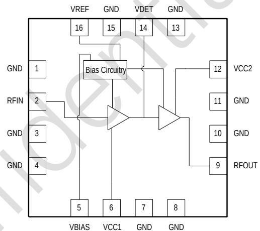
Figure 2. GSM0824 Function Block Diagram
