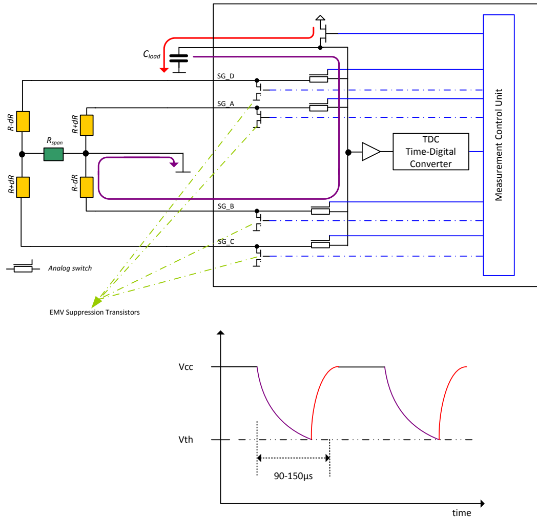
Figure 3-32: PS09 with EMV transistors
