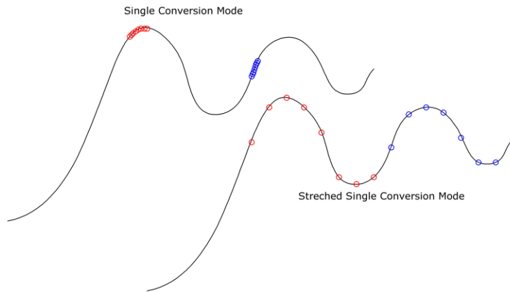
Figure 3-20: Undersampling
