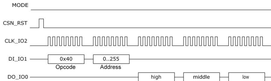
Figure 4-11: RAM read access
