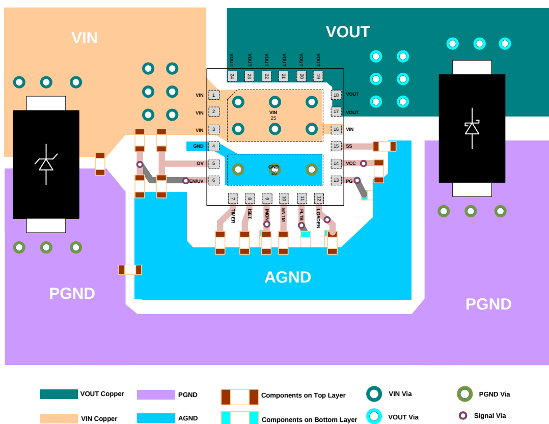
Figure 12: Recommended PCB Layout
