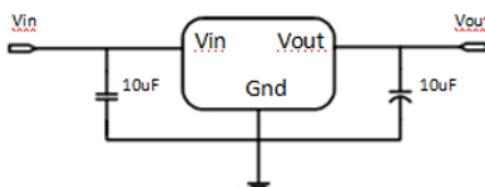
Application circuit of 1117A fixed version
