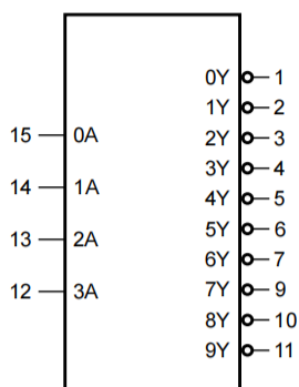
Figure 1. Logic symbol
