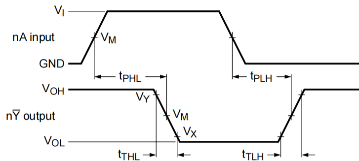
Figure 6. Input ( nA ) to output ( n\bar{Y} ) propagation delays and output transition times
