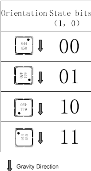
FIGURE 3-1 Device Orientation
