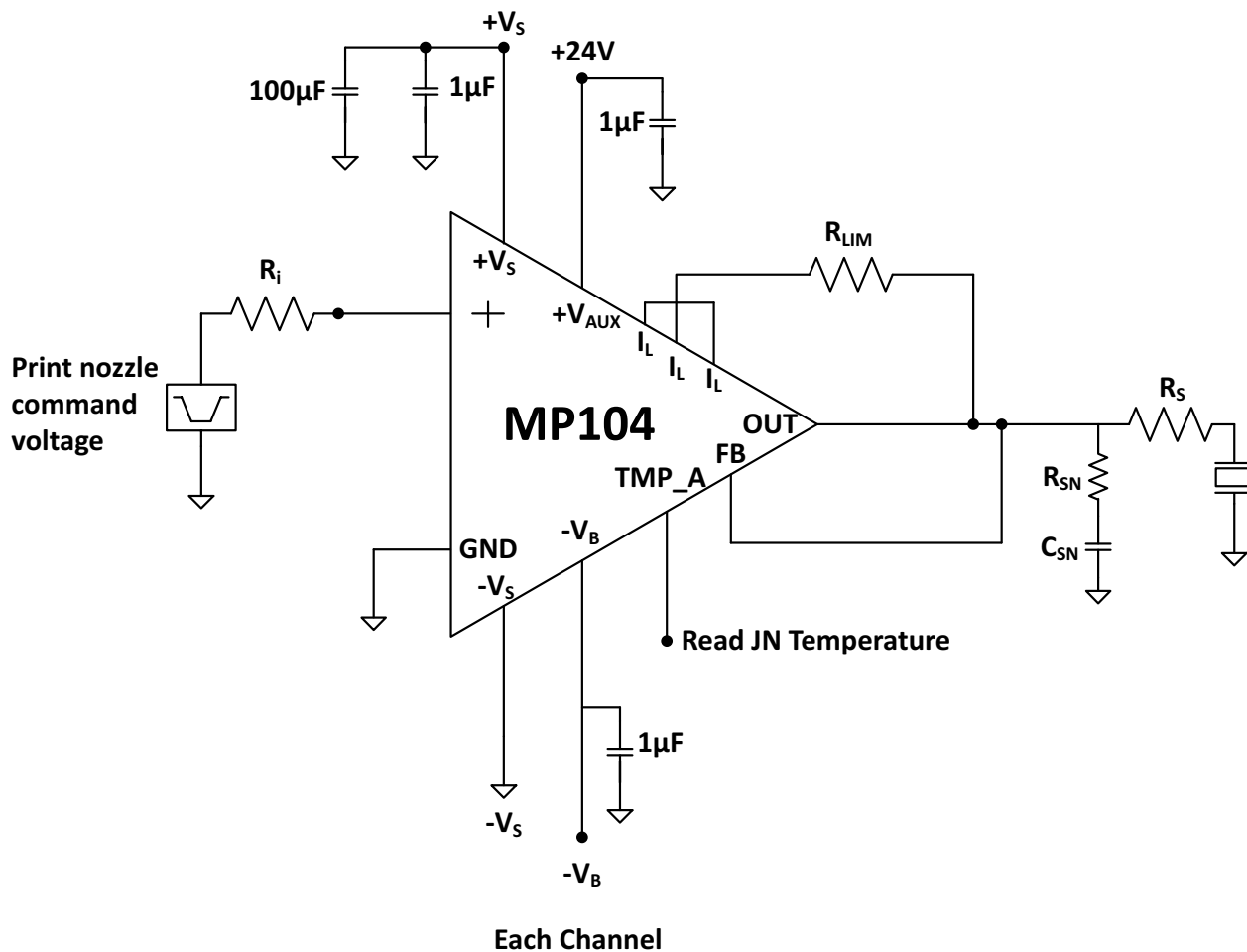
Figure 2: Typical Connection
