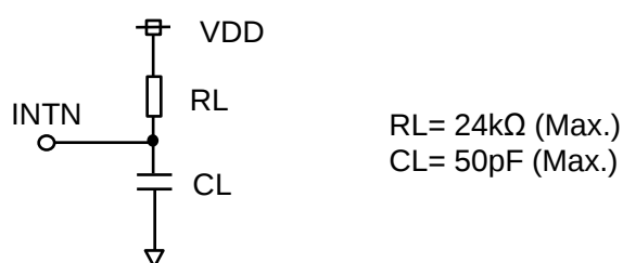
Figure 9.2. INTN Output Load Circuit
