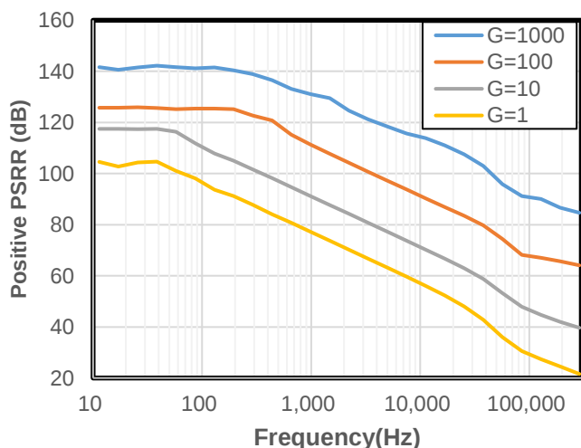
Figure 3 Positive PSRR Vs. Frequency
