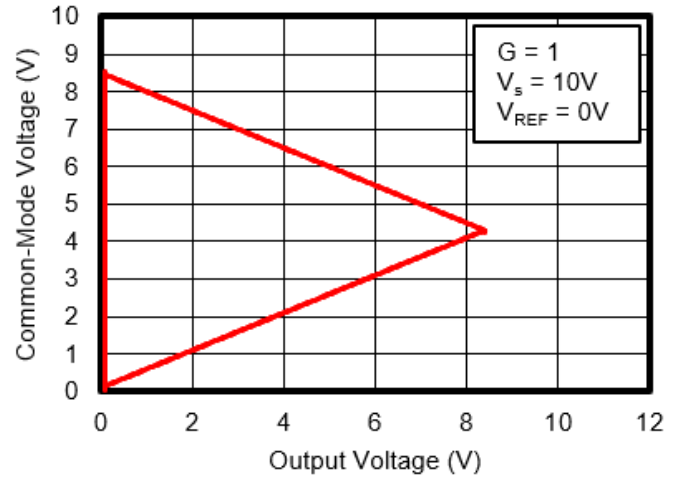
Figure 38 Input Common-Mode Range vs. Output Voltage
