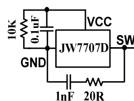
RC Snubber circuit
